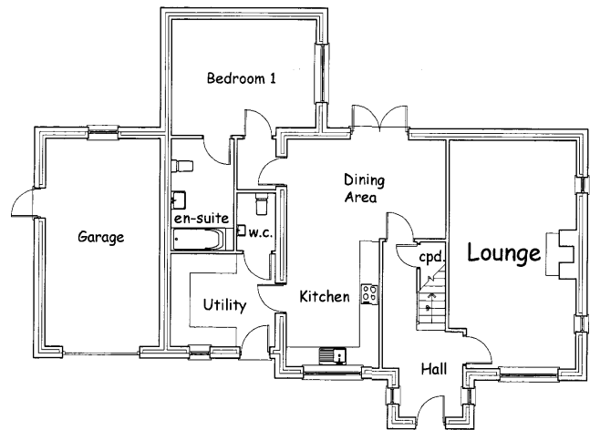
Plot 1 Ground Floor Plan
