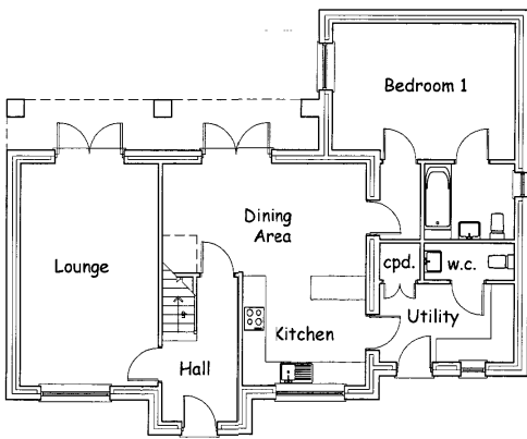
Plot 2 Ground Floor Plan
